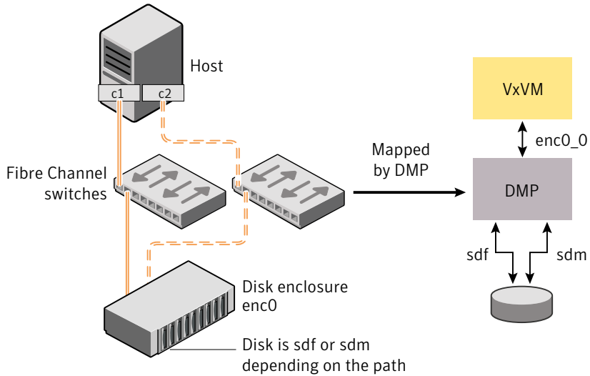
Figure 5-2 Example of multi-pathing for a disk enclosure in a SAN environment
