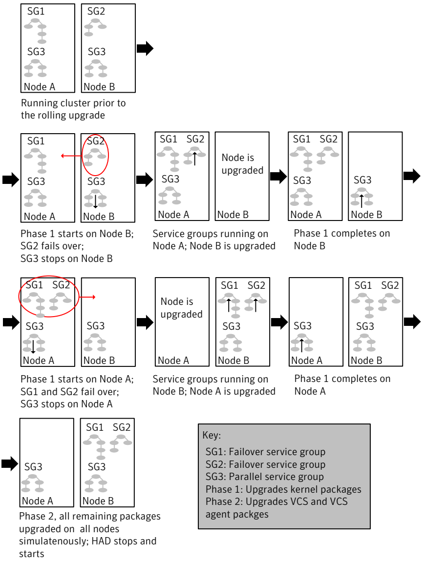
Figure 15-1 Example of the installer performing a rolling upgrade
