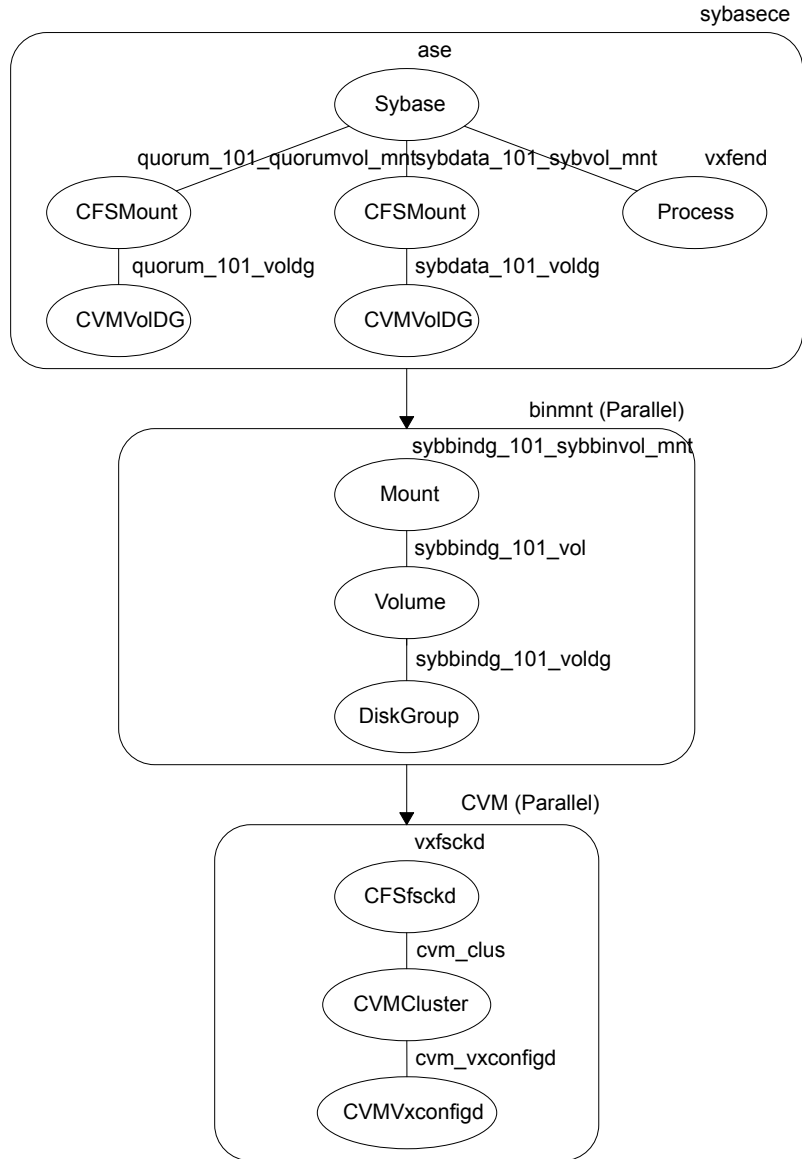
Figure 17-2 displays the service group dependencies for an SF Sybase CE configuration on shared disk group with CFS.
