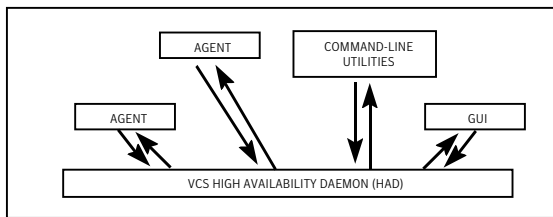
Figure 9-1 Basic communication on a single VCS system
