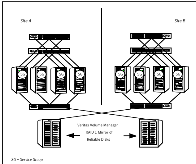
Figure 2-9 Campus shared storage cluster
