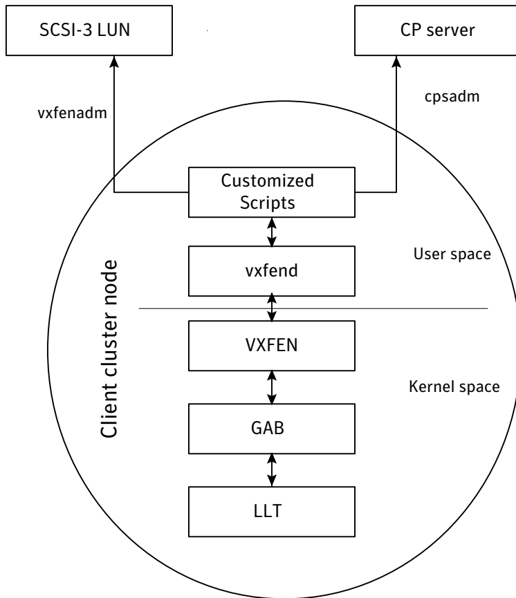
Figure 9-6 Customized fencing
