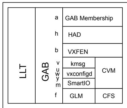
Figure 1-6 Low-level communication
