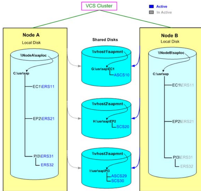
Figure 3-1 Typical SAP system installation (using multiple sapmnt file shares) on a Windows Server 2008 system under VCS environment
