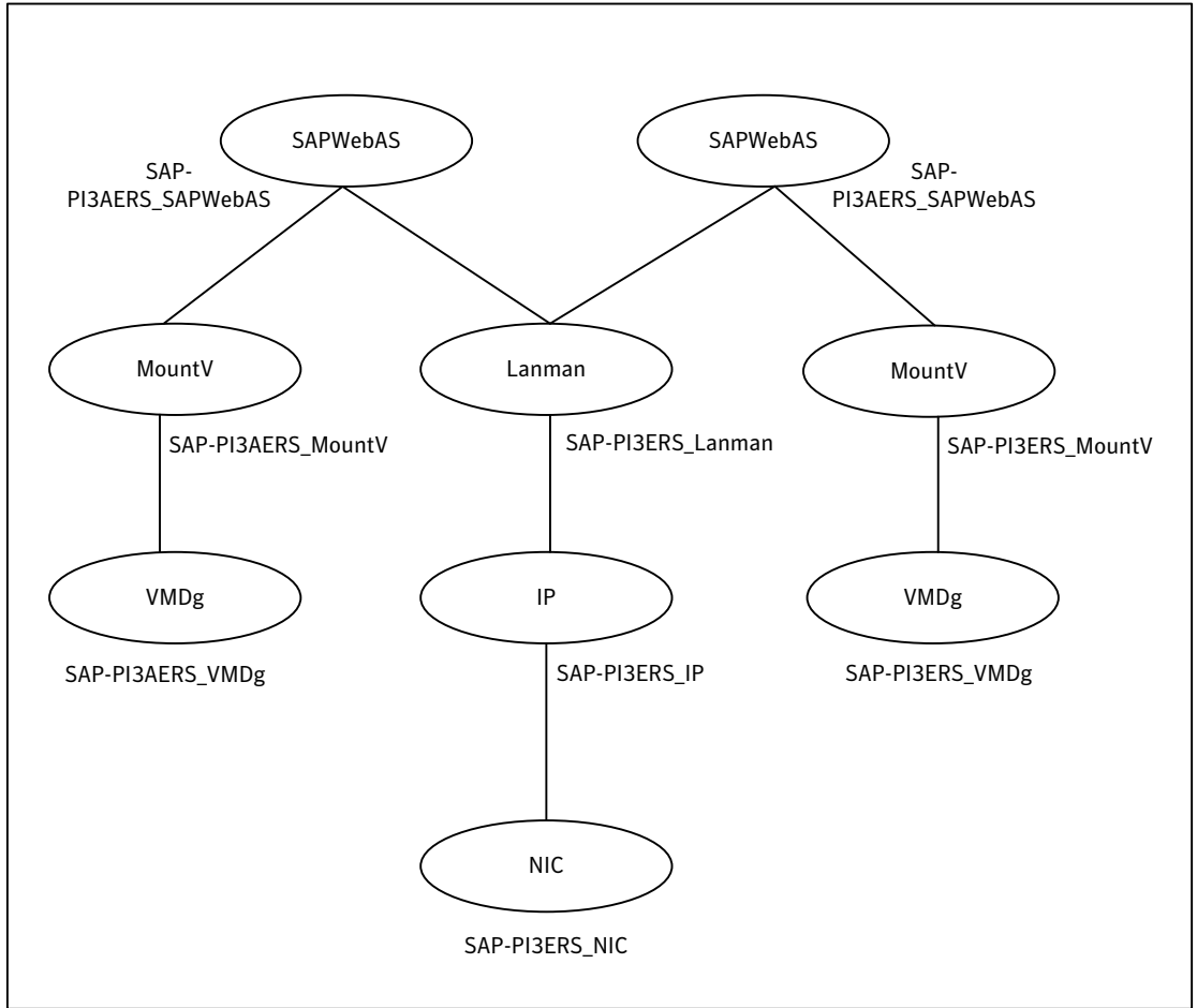
Figure A-7 Sample resource group dependency for SAP Enqueue Replication Server Instances service group for Add-In installation Usage Type
