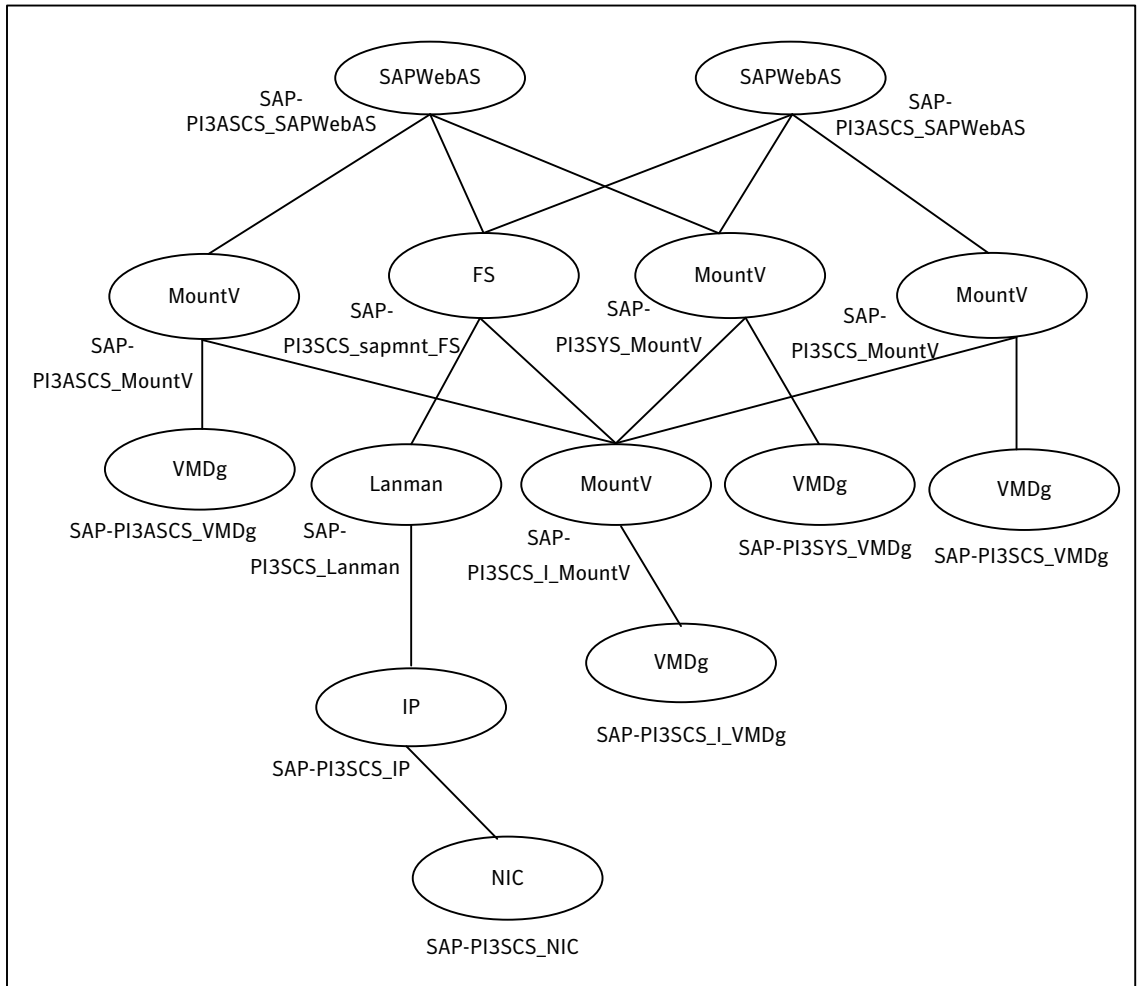
Figure A-6 Sample resource dependency diagram for SAP Central Services Instances service group for Add-In installation Usage Type on a Windows 2008 Server
