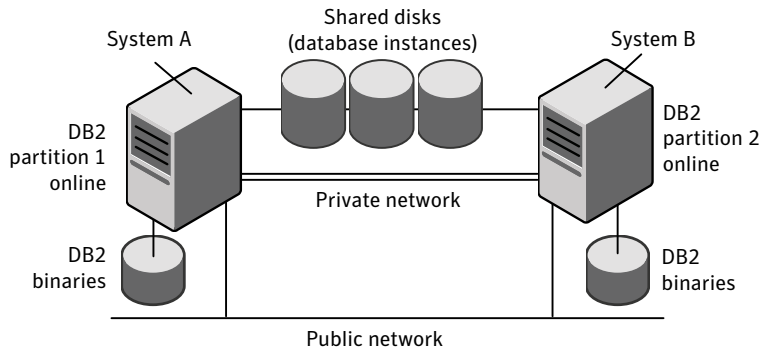
Figure 1-2 DB2 installation with an MPP configuration
