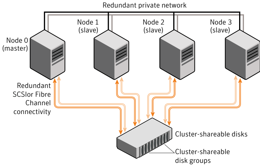
Figure 5-1 Example of a 4-node CVM cluster
