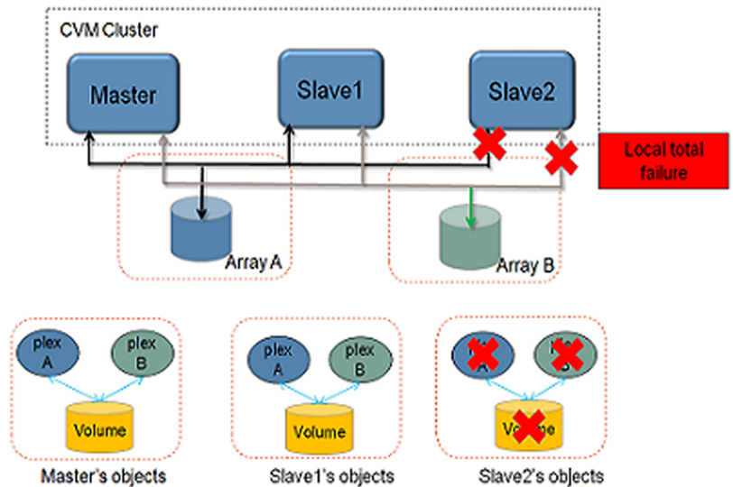
Figure 5-10 Local total failure - policy independent
