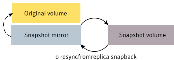
Figure 23-8 Resynchronizing an original volume from a snapshot
