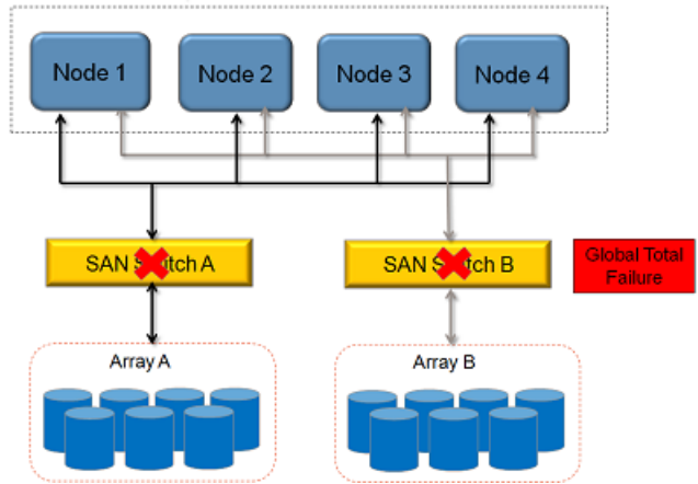
Figure 5-9 Global total failure - policy independent
