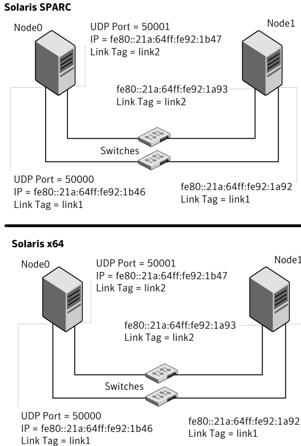
Figure K-3 A typical configuration of direct-attached links that use LLT over UDP
