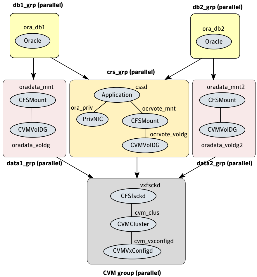
Figure 24-3 Service group configuration with the VCS Oracle agent (alternate configuration)
