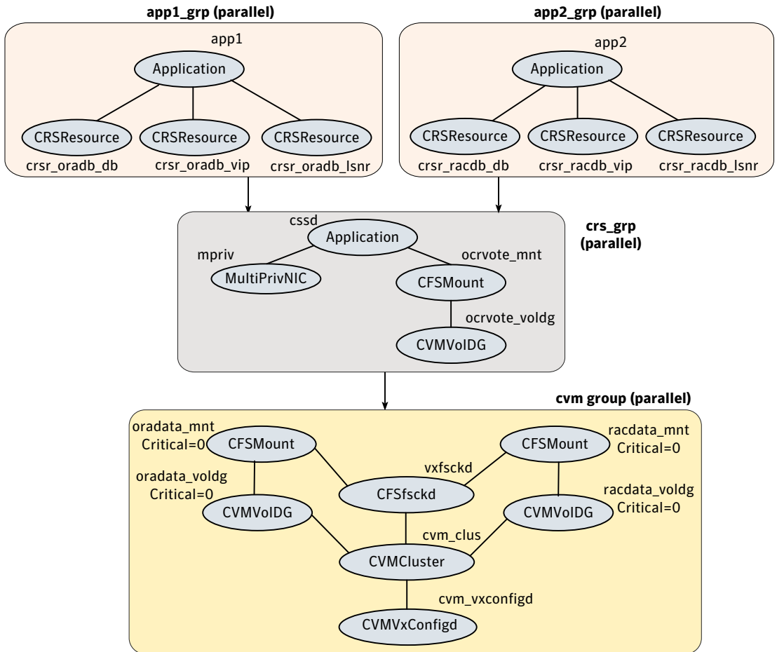
Figure D-4 Service group configuration for sfrac04_main.cf file
