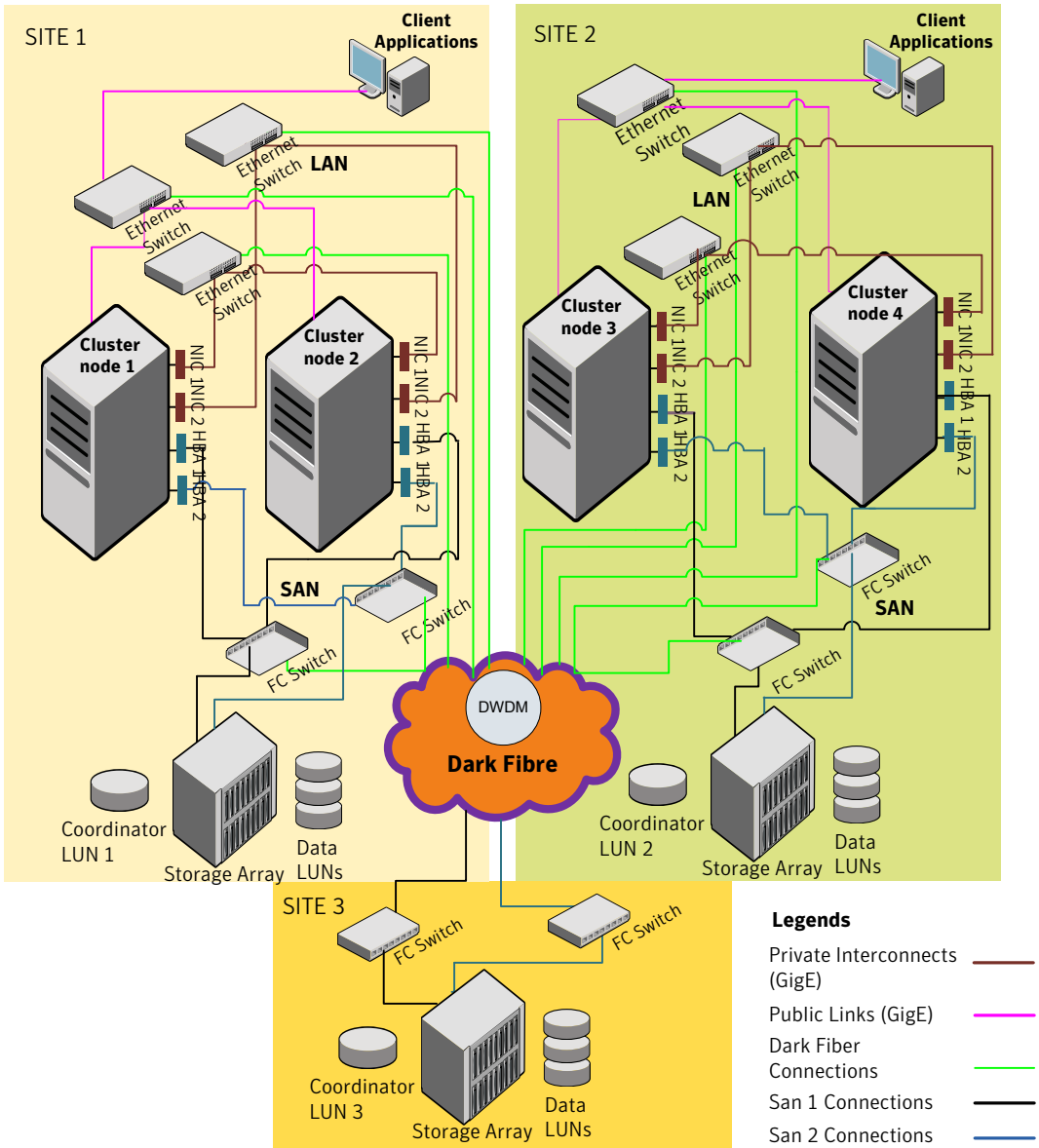
Figure 1-4 Basic campus cluster setup
