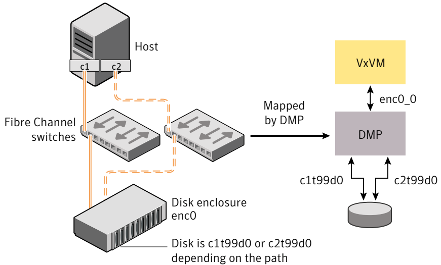
Figure 5-2 Example of multi-pathing for a disk enclosure in a SAN environment
