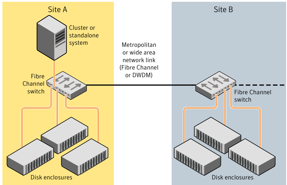
Figure 19-3 Example of a two-site configuration with remote storage only
