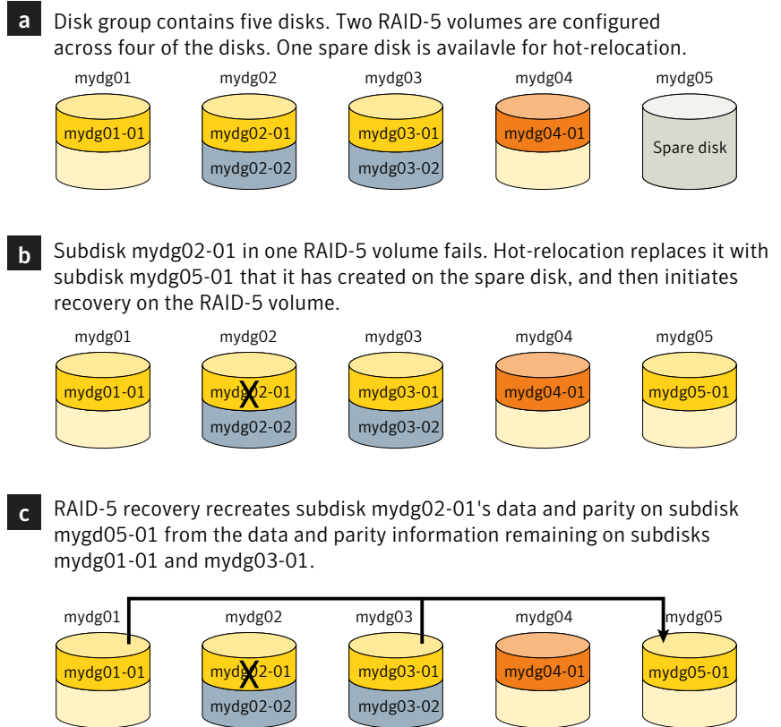
Figure 36-1 Example of hot-relocation for a subdisk in a RAID-5 volume
