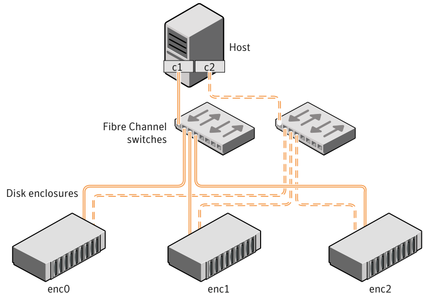
Figure 5-4 Example HA configuration using multiple switches to provide redundant loop access
