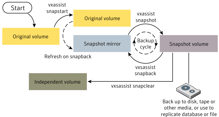
Figure 25-1 Third-mirror snapshot creation and usage
