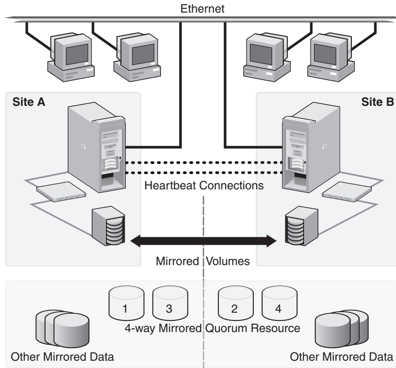
Figure 3-2 Typical campus clustering configuration
